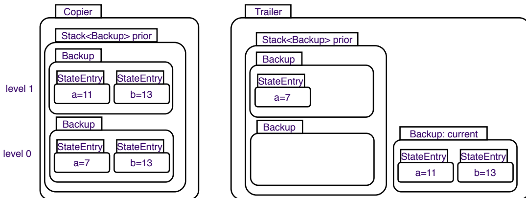
Fig. 3: Illustration of the differences between Copier and Trailer related to example given in Listing 20.
